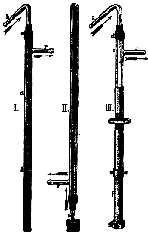
FIG. 23.—MEYER'S THERMO-REGULATOR.
